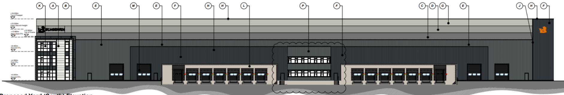
Proposed Yard (South) Elevation
